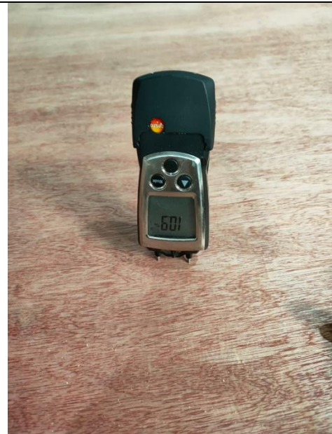
Moisture content test: 10.9%
